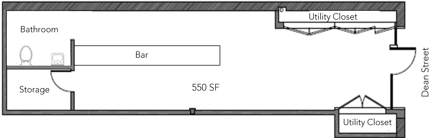
Floor Plan
